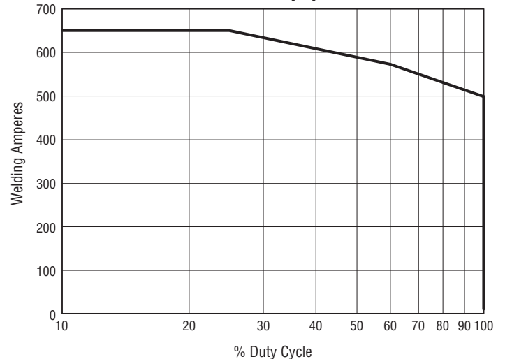
Deltaweld 500 Duty Cycle Chart
